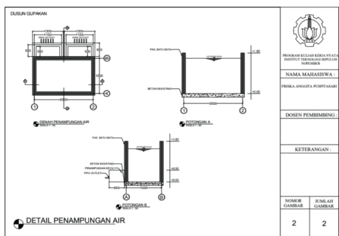
Gambar 8. Detail Engineering Desain Desa Nawangan Titik 2
