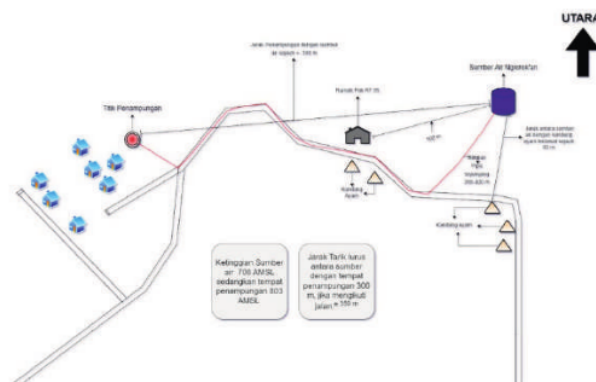
Gambar 11. Detail Engineering Desain Desa Tegalombo
