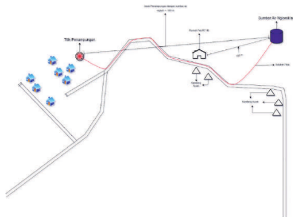
Gambar 10. Detail Engineering Desain Desa Tegalombo
