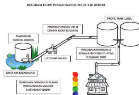
Gambar 6. Detail Engineering Desain Desa Kasihan
