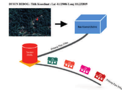
Gambar 4. Detail Engineering Desain Dusun bedog Desa Kalikuning
