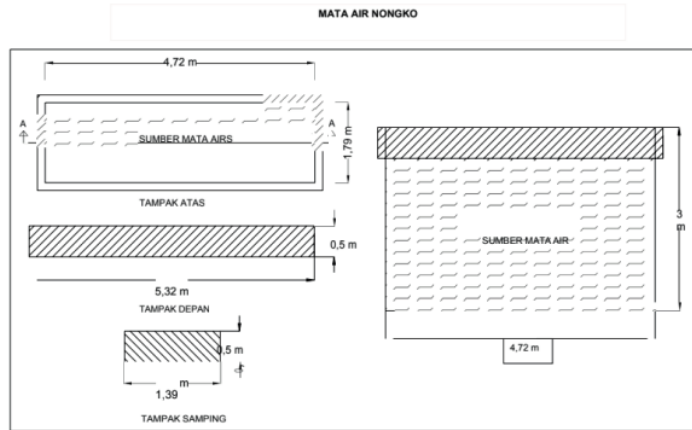
Gambar 7. Detail Engineering Desain Desa Petungsinarang
