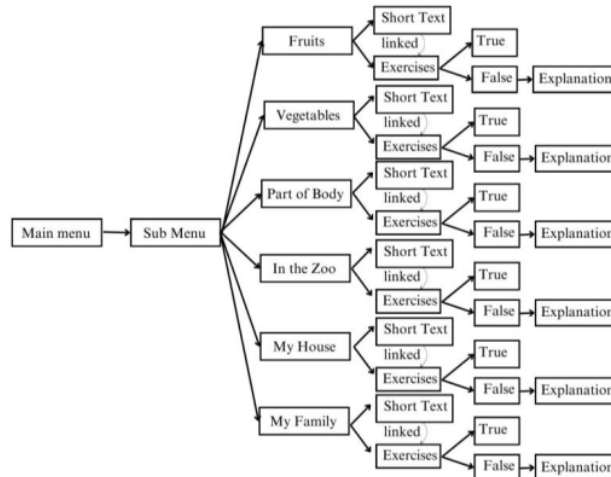
Figure 7: Contoh Workflow Aplikasi
